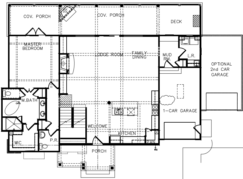
1st FLOOR PLAN 1575 SQ. FT. GARAGE 254 SQ. FT.
