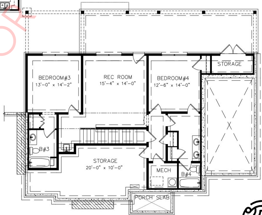
TERRACE PLAN 1076 SQ. FT.
