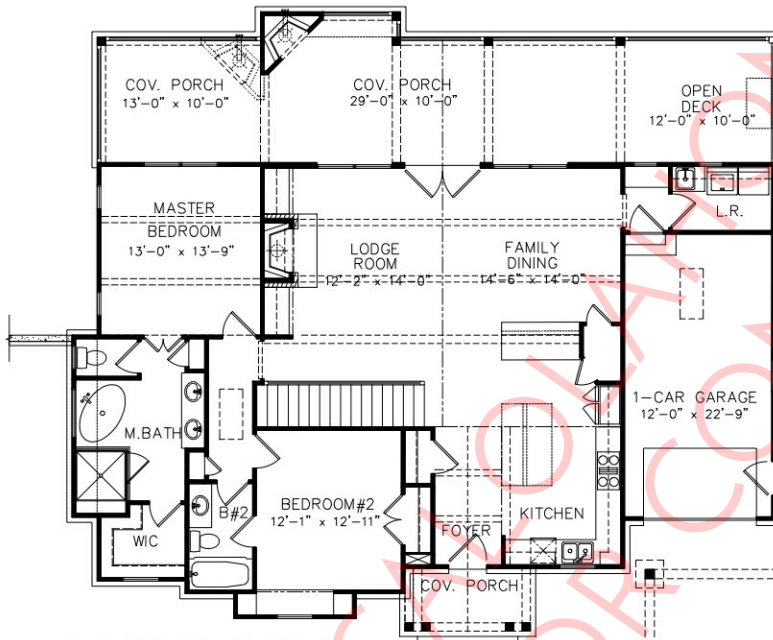
1st FLOOR PLAN 1517 SQ. FT. GARAGE 273 SQ. FT.
