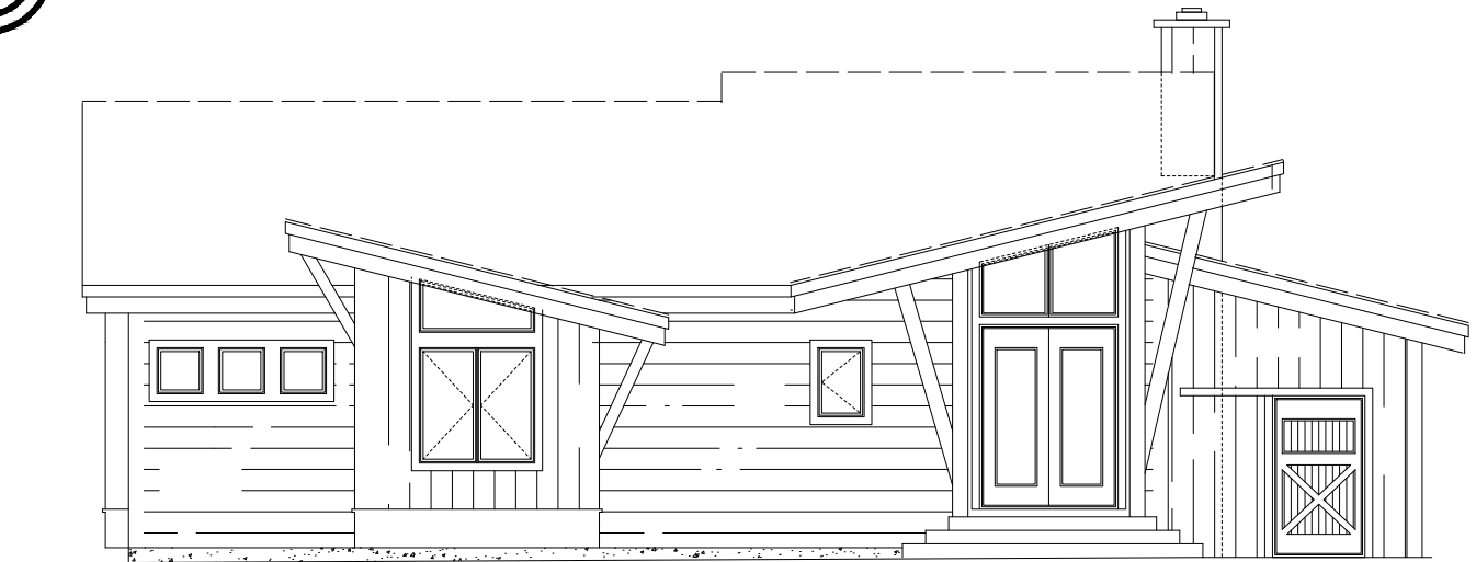
FRONT ELEVATION
