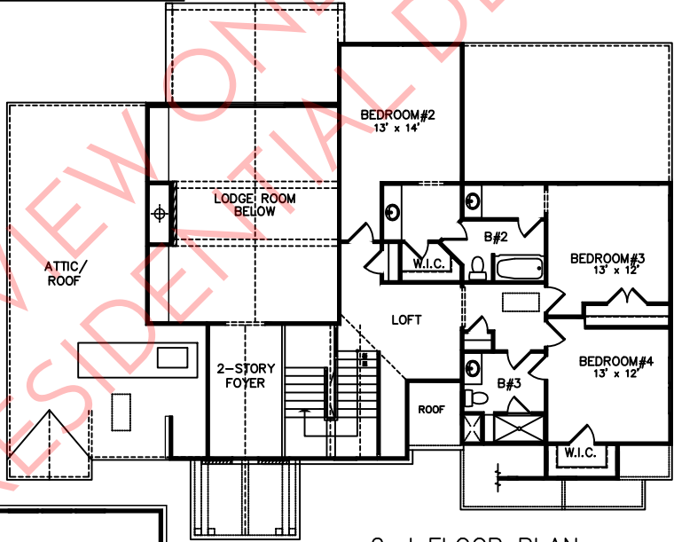
2nd FLOOR PLAN 1,031 SQ. FT.
