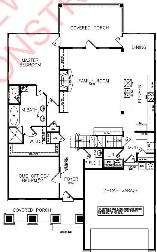
1st FLOOR PLAN 1,636 SQ. FT. GARAGE: 461 SQ. FT.
