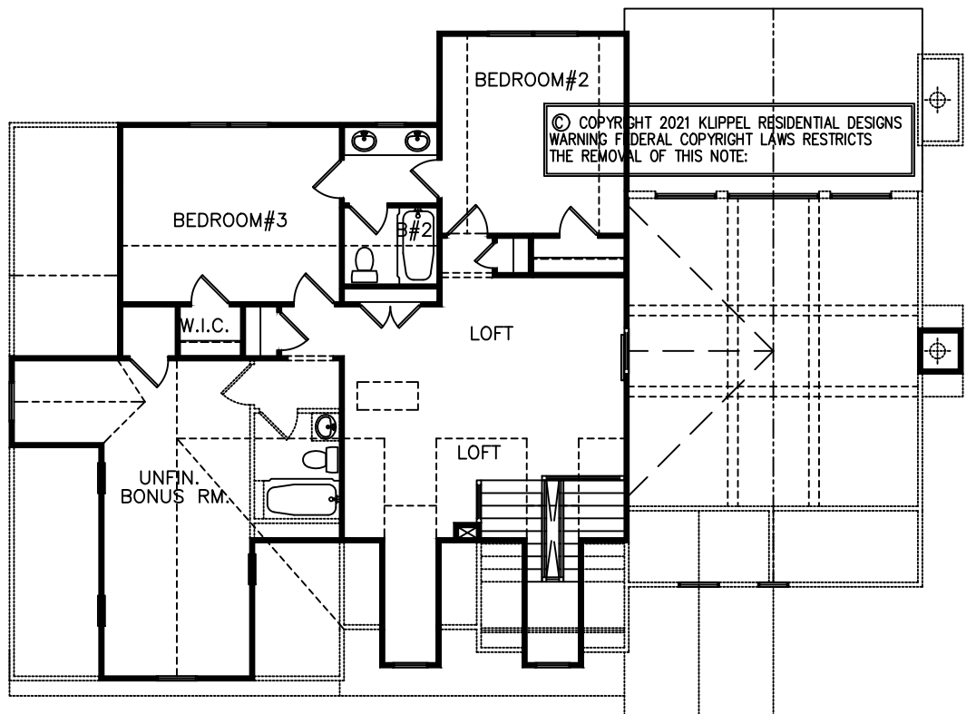
2nd FLOOR PLAN 806 SQ. FT. BONUS 332 SQ. FT.
